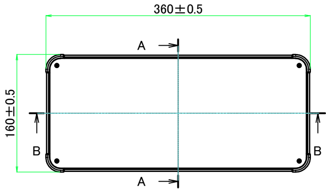
E view
